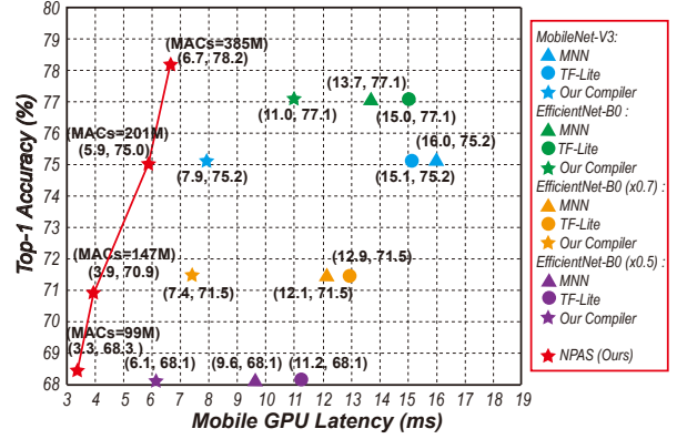
Figure 6. Accuracy vs. Latency comparison on mobile GPU.
