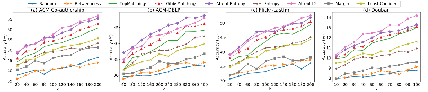
Figure 4: Alignment accuracy vs. # queries in four alignment scenarios using IsoRank algorithm. The top two solid lines represent the proposed ATTENT-Entropy and ATTENT-L2 respectively. Best viewed in color.
