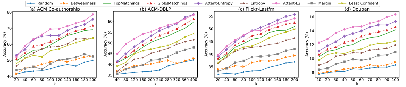
Figure 3: Alignment accuracy vs. # queries in four alignment scenarios using NetAlign algorithm. The top two solid lines represent the proposed ATTENT-Entropy and ATTENT-L2 respectively. Best viewed in color.
