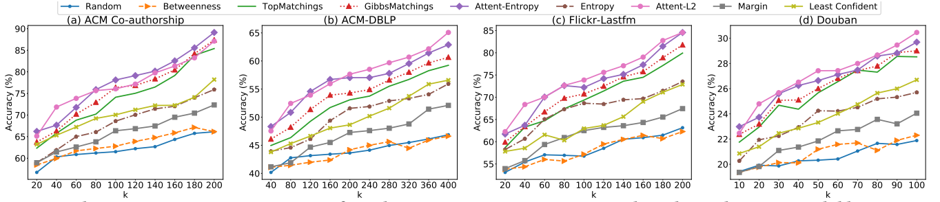
Figure 2: Alignment accuracy vs. # queries in four alignment scenarios using FINAL algorithm. The top two solid lines represent the proposed ATTENT-Entropy and ATTENT-L2 respectively. Best viewed in color.
