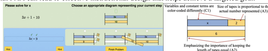
Figure 3. Our ITS with diagrammatic-self-explanation (left). Figure 4. The design of the tape diagrams used in the ITS (right).
