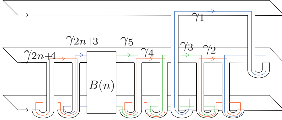
FIGURE 4. The Seifert surface T_n of K_n . The oriented curves \gamma_1, \dots, \gamma_{2n+4} generate H_1(T_n) .
