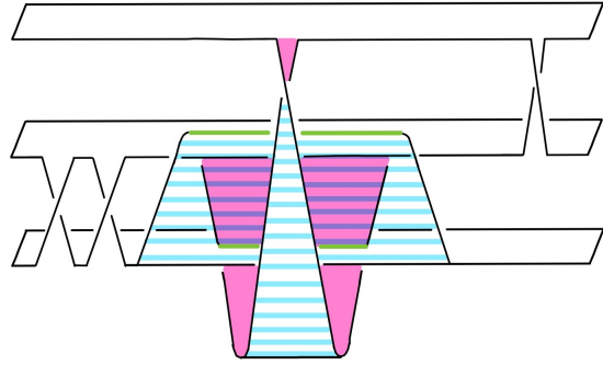
FIGURE 7. S_1 with colored band
