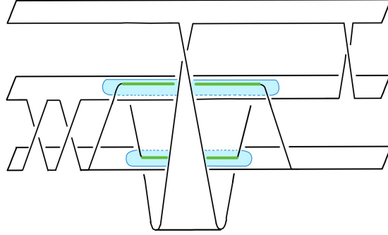
FIGURE 6. S_1 with ribbon intersections
