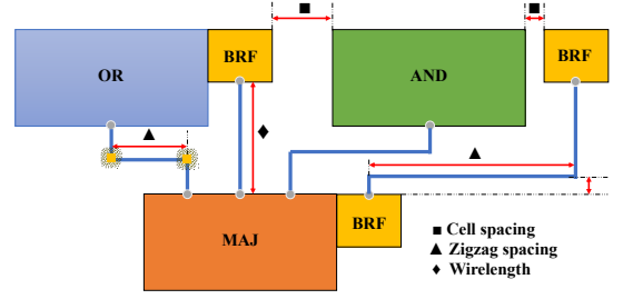
Fig. 3: The Illustration of spacing constraints in the AQFP placement with the detail of interconnect via.
