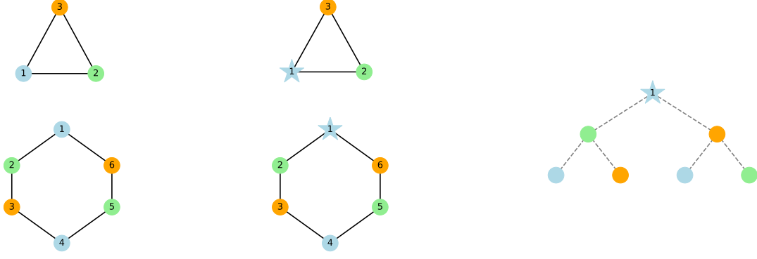
Figure 4: An illustration of rooted graphs and rooted aggregation trees. Left: a pair of graphs, G and G' . Center: the rooted graphs of 1 in G and G' , G^{[1]} and G'^{[1]} . Right: the rooted aggregation tree that both G^{[1]} and G'^{[1]} correspond to.
