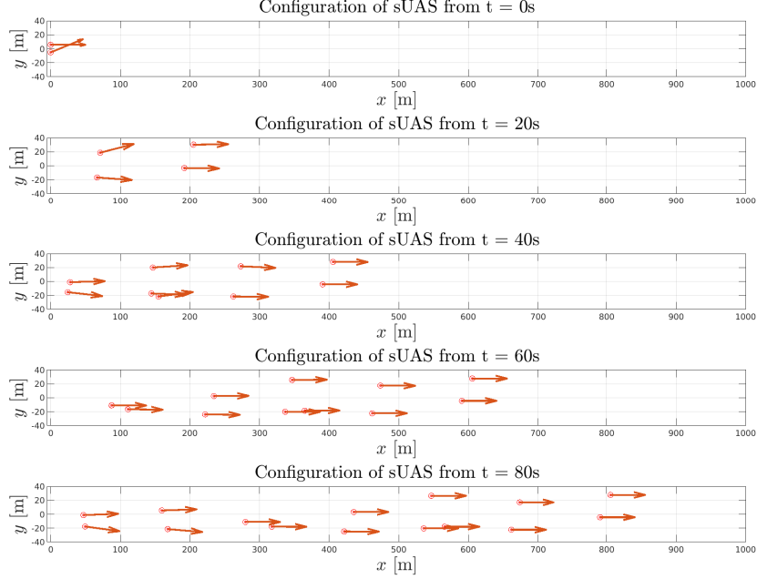
Figure 2: Configurations of sUAS in every 20s after the entry of a new group of sUAS's
