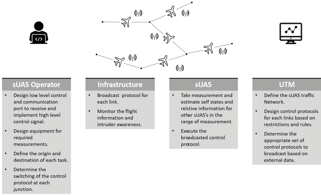
Figure 1: Proposed UTM framework
