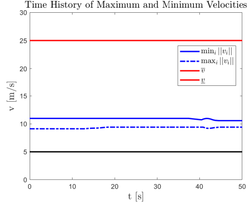
Figure 4: Time history of Minimum Velocity and Maximum Velocity
