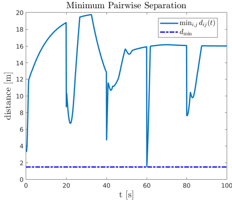
Figure 3: Minimum Pairwise Separation
