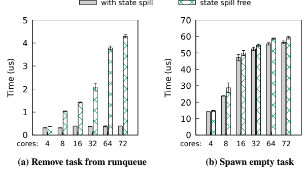
Figure 4: (a) The time to remove a task from the runqueue(s) increases when eliminating runqueue states from the task struct, but is minor in the worst realistic case of (b) spawning an empty task.
