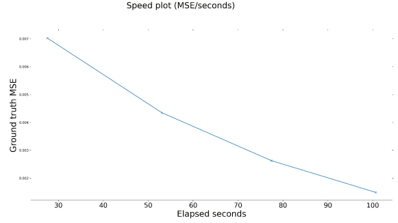
Figure 6. Speed plot (MSE / elapsed seconds) for the task of inversion. We use a single V100 GPU. We run 300 optimization steps per layer. The leftmost point corresponds to CSGM, i.e. we optimize over only the first layer. For each other point, we also optimize over the input space of a layer one level deeper compared to the previous point, e.g. the rightmost point corresponds to 1200 optimization steps (300 for each one of the first four layers).
