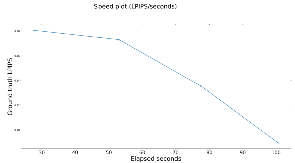
Figure 7. Speed plot (LPIPS / elapsed seconds) for the task of inversion. We use a single V100 GPU. We run 300 optimization steps per layer. The leftmost point corresponds to CSGM, i.e. we optimize over only the first layer. For each other point, we also optimize over the input space of a layer one level deeper compared to the previous point, e.g. the rightmost point corresponds to 1200 optimization steps (300 for each one of the first four layers).
