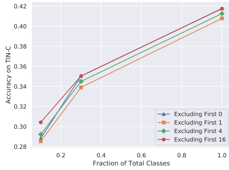
(c) TinyImageNet-C Excluding First Layers
