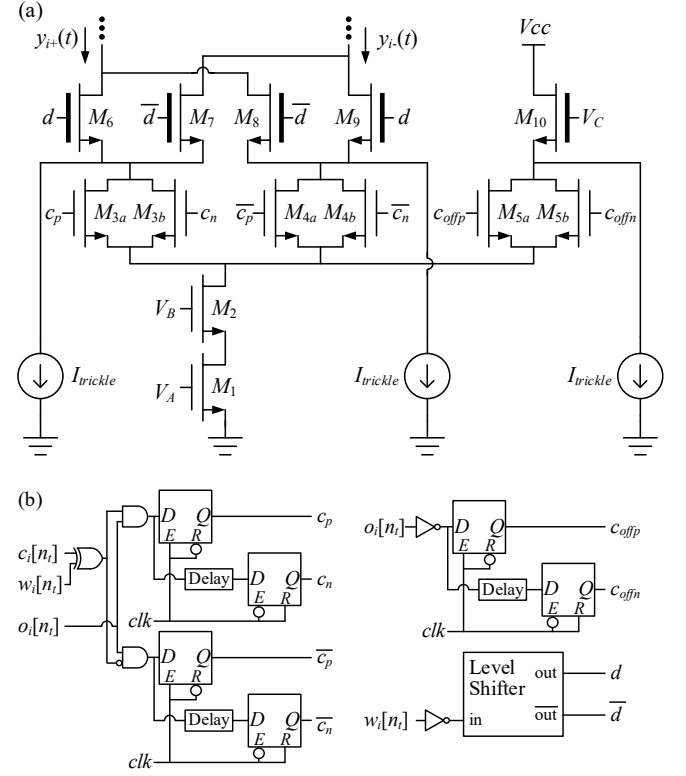
Fig. 4 ISI scrambling 1-bit DAC implementation, (a) current-steering cell, (b) switch driver.
