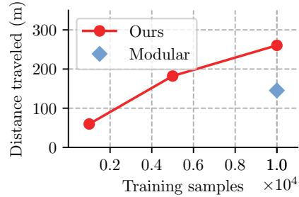
Fig. 5: Performance at different amounts of target-domain training data.
