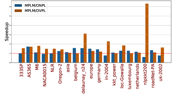
Figure 7: Speedup of ONPL and OVPL over MPLM on the SkylakeX (36 threads)
