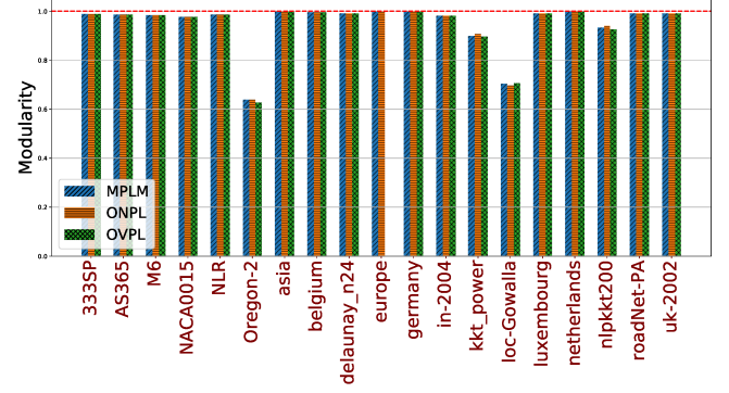
(b) Modularity of MPLM, ONPL, and OVPL on Cascade Lake(48 threads).
