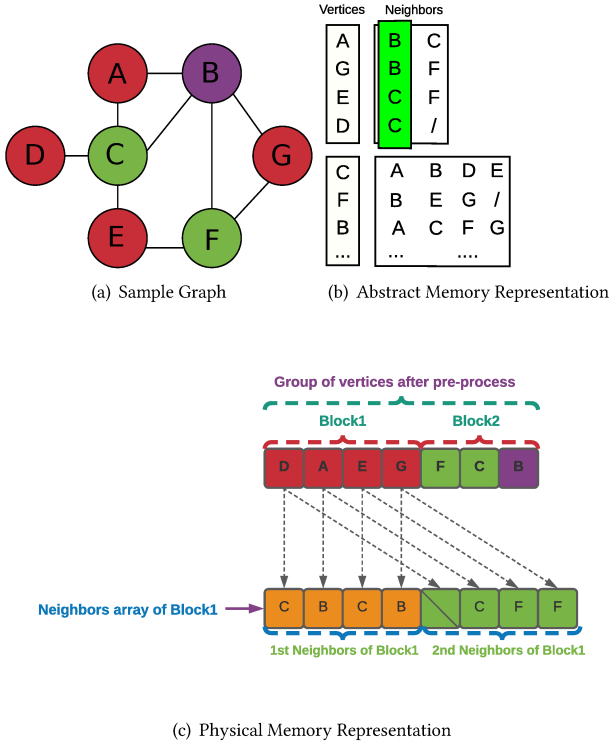
Figure 3: OVPL reorders the graph using a graph coloring methods and structure it in blocks of vertices so that the neighbors of the vertices of a block can be loaded in a vector (sketched in green) simultaneously.
