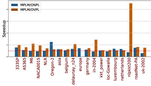
Figure 6: Speedup of ONPL and OVPL over MPLM on the Cascade Lake (48 threads)
