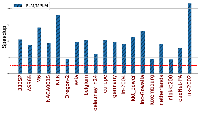
(a) PLM vs MPLM speedup on the Cascade Lake(48 threads).
