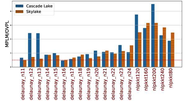
Figure 8: Speedup of OVPL over MPLM for the selected graphs where many vertices have degrees close to the average on both architectures.
