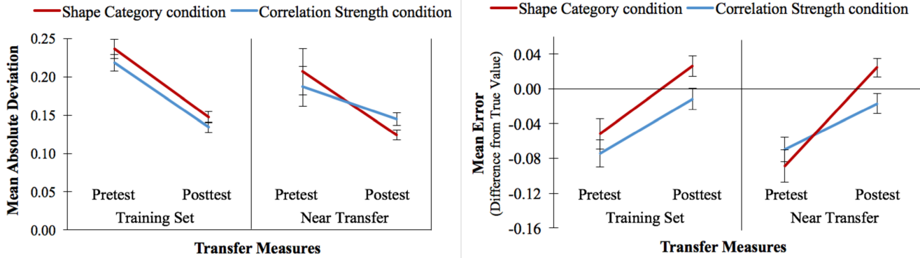
Figure 2. (Left) Improvements in mean absolute deviation on training set and near transfer items from pretest to posttest. (Right) Improvements in mean error on training set and near transfer items from pretest to posttest. Error bars represent +/- 1 standard error.
