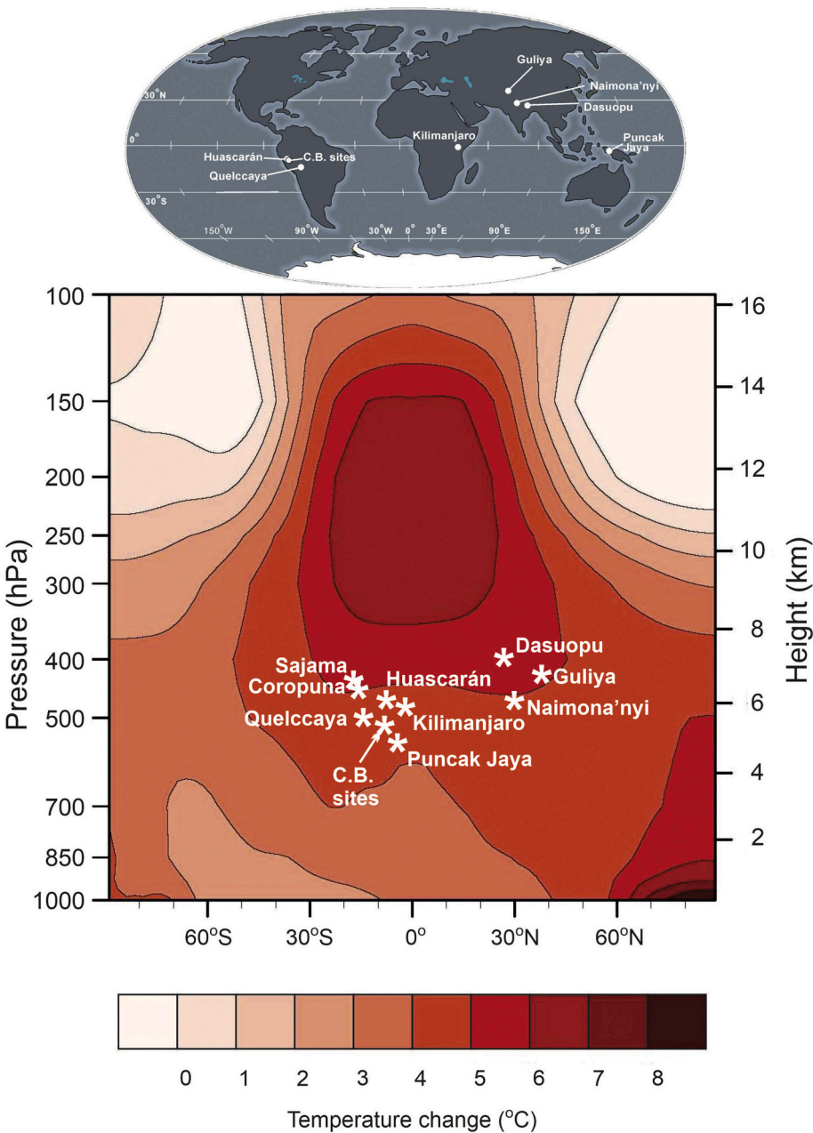
Fig. 11. Projected zonal annual temperature changes with height in the atmosphere between 2000 and 2009 and 2090–2099. The multi-model mean for RCP 8.5 was calculated by KNMI Climate Explorer using CMIP5 data from https://esgf-node.llnl.gov/search/cmip5/ . Latitudes and altitudes are shown for the tropical and mid-latitude alpine glaciers from which ice cores discussed in the paper were drilled. “C.B. sites” indicates the alpine glaciers (Hualcán, Pucallirca, Copap, and Caullaraju) drilled in the Cordillera Blanca, in addition to Huascarán (see Fig. 2, inset).
