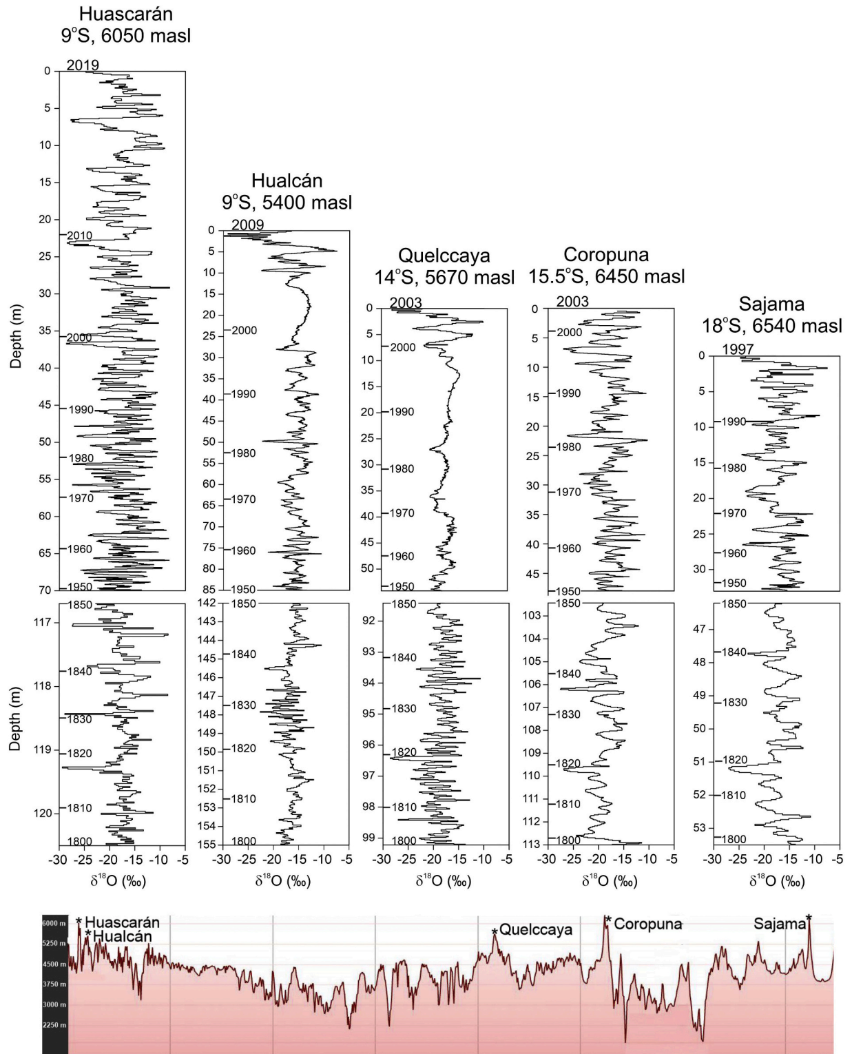
Fig. 4. \delta^{18}\text{O} profiles from five ice cores drilled in the Peruvian Andes and on the Altiplano of Bolivia, arranged from north to south. The \delta^{18}\text{O} sample data are illustrated in two time slices, 1800 to 1850 CE and 1950 CE to the top of each record, and the mean \delta^{18}\text{O} values for these two periods are shown for each record in Table 1. Timescale development is discussed for: Huascarán in Thompson et al. (1995) (and updated with \delta^{18}\text{O} data from a core drilled in 2019), Quelccaya in Thompson et al. (1986, 2013), Coropuna in Thompson et al. (2018a), and Sajama in Thompson et al. (1998). The elevation profile below (Google Earth Pro) shows the topography from north to south (black dashed line in Fig. 2) and the relative elevations of the glaciers in this section of the outer tropical Andes. The year of drilling is shown at the top of each core. The analytical error of \delta^{18}\text{O} is \pm 0.2\text{‰} .
