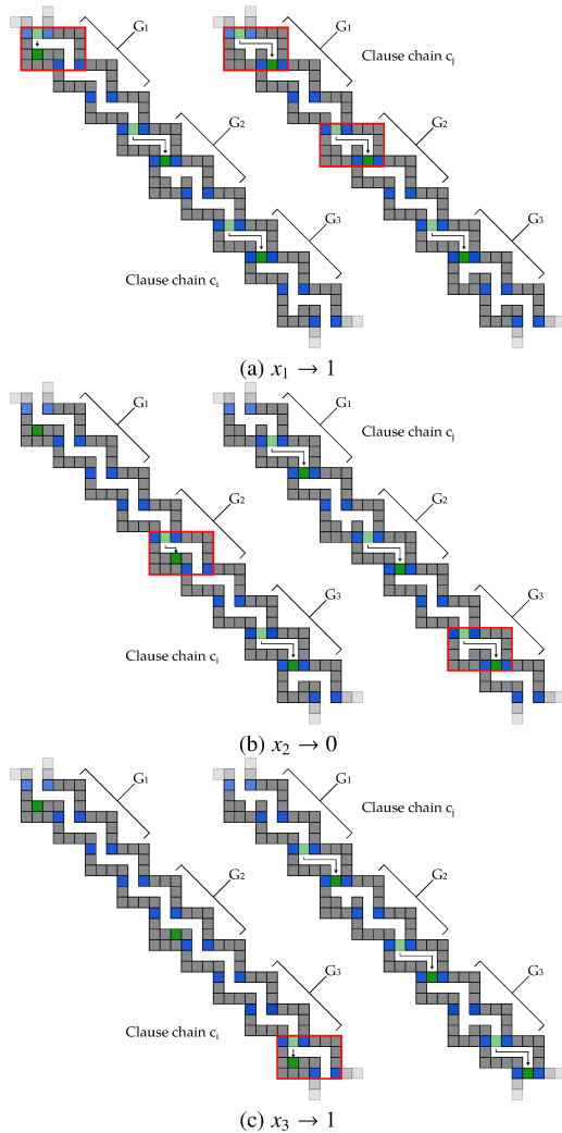
Fig. 5 Visualization of two clause chains c_i = (x_1 \vee \neg x_2 \vee x_3) , c_j = (\neg x_1 \vee \neg x_1 \vee x_2) for X = \{x_1, x_2, x_3\} during the first phase. (a) Assigning the variable x_1 to true value is done by the step sequence \langle S, 3E, 2S \rangle , which makes all other tiles in the clauses chains and assignment section move to the next gadget. (b) Assigning the value false to the variable x_2 is done by the sequence \langle E, S, 3E, 2S \rangle . (c) By performing the true sequence again, the variable x_3 can be assigned some truth value as well.
