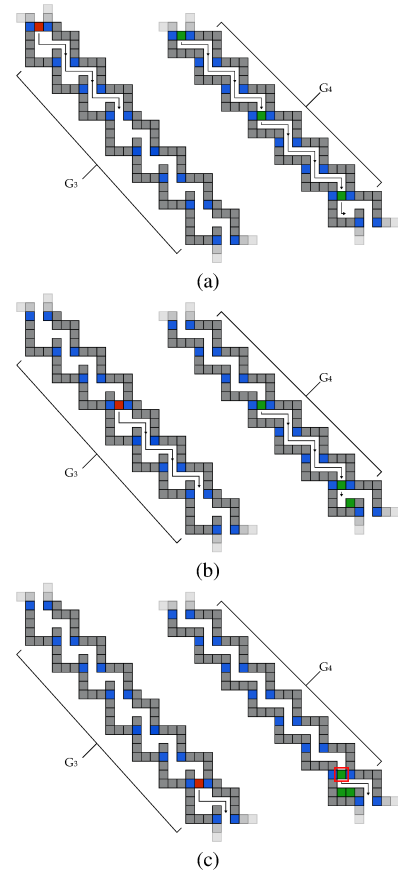
Fig. 6 During the second phase, unconfined literal tiles are forced inside the Notch gadget of the fourth chain of their corresponding clause chain. Unsatisfied clause chains export one too many literal tiles, as shown in (c).
