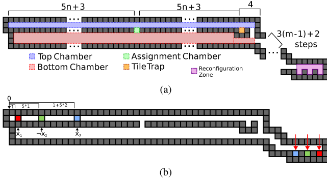
Fig. 7 (a) 3 SAT clause gadget, where n is the total number of unique variables, and m indicates that this clause is the m th clause in the formula. (b) Example of variable placement for clause (x_1 \vee \neg x_2 \vee x_3) in a 5 variable formula. Goal locations indicated by red arrows.
