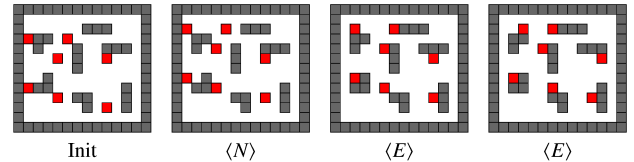
Fig. 1 An example step sequence. The initial board configuration followed by the resulting configurations after an N step, E step, and then final E step. So, the sequence to get from the initial state to the final state in this figure is \langle N, 2E \rangle .
