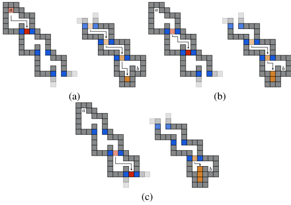
Fig. 4 Illustration of validation tiles entering the Goal gadget as truth assignments are made. In (a) and (c), true assignments are made, showing the start and end location of the tiles. In (b), a false assignment was made, showing how the validation tiles are still placed outside of location b .
