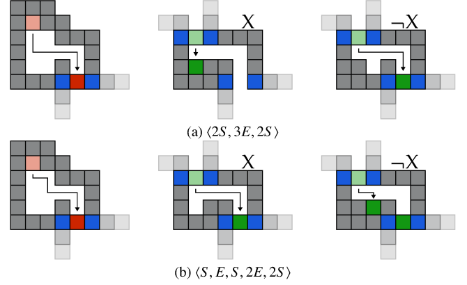
Fig. 3 Assigning (a) true or (b) false to some variable x . Setting a literal to true is done by confining its corresponding literal tile within a Positive or Negative gadget.
