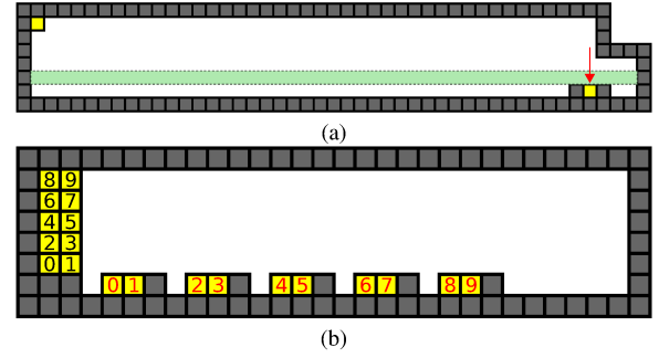
Fig. 9 (a) Example of south limiter tile placement in a 5 variable formula. Goal location indicated by red arrow. Post assignment zone highlighted in green. (b) Example of south forcer tile placement in a 5 variable formula. Goal location indicated by red labels.
