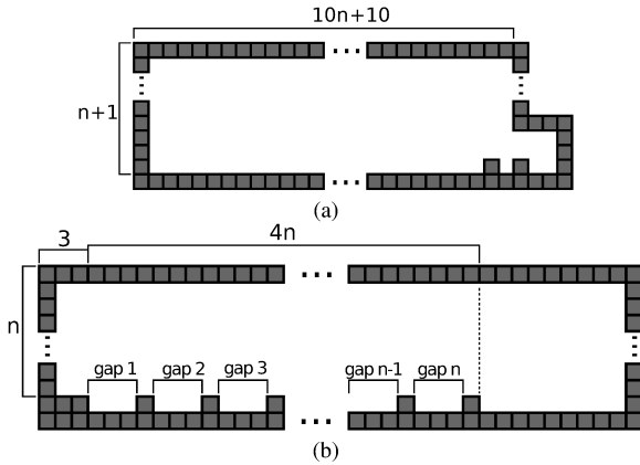
Fig. 8 (a) South Limiter: Limits the amount of south steps made before all variables have been assigned. (b) South Forcer: Forces the user to make south steps at specific times
