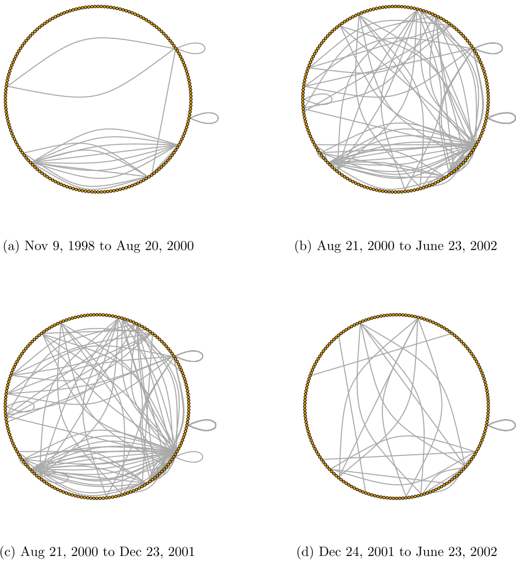
FIG. 11. Estimated Fréchet means of weekly network adjacency matrices for the time periods as indicated.
