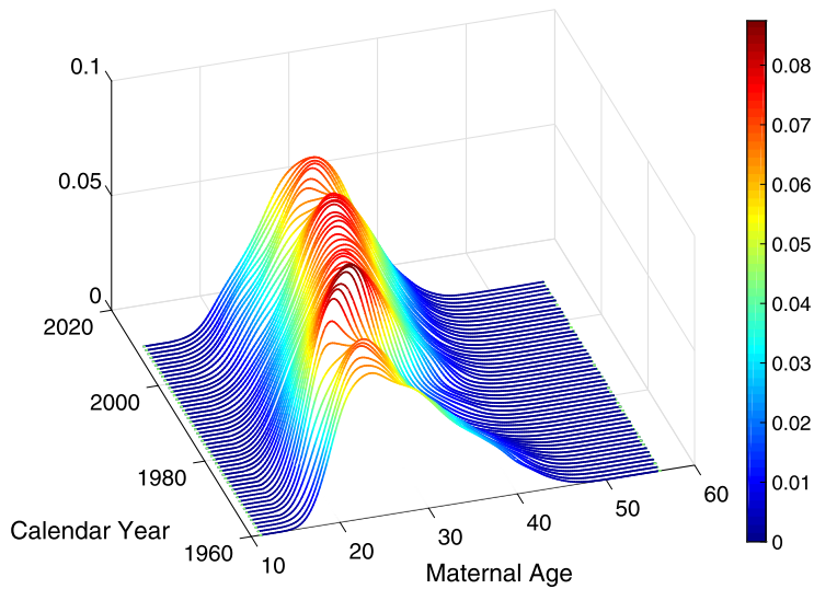
FIG. 6. Yearly maternal age distributions represented as density functions for the age interval [12, 55] during the time period 1960 to 2010 for the Finnish fertility data.
