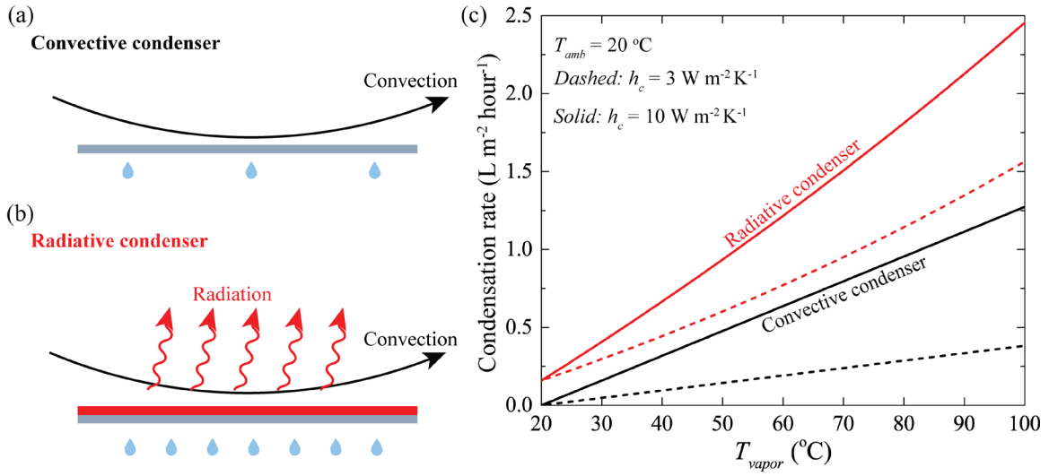
Figure 2. Performances of convective condenser and radiative condenser. (a) and (b) Schematic of a convective condenser (a) and our radiative condenser (b). The convective condenser dissipates heat through only convection, while the radiative condenser dissipates heat through both convection and radiation. (c) Theoretically calculated condensation rates of the convective (black) and radiative condenser (red), assuming an ambient temperature of 20^{\circ}\text{C} . To analyze the theoretical upper bound of condensation rate, we assume a relative humidity of 100% throughout our calculation.
