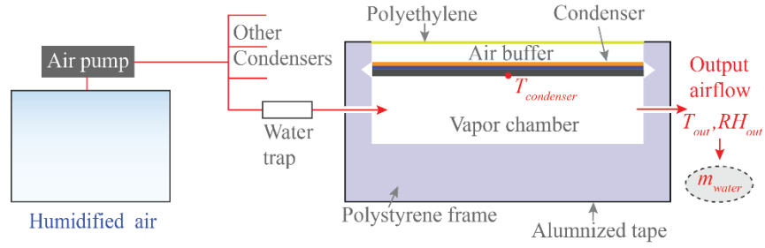
Figure 5. Schematic of the outdoor experimental setup for condensation. Humidified air was pumped into all condensers (the convective, blackbody, commercial and radiative condensers) at the same rate. All airflow into the condensers were filtered by a water trap to remove water droplets. The humidified air then passed through the condensing chamber and then exit the chamber through an outlet. The temperature T_{out} and relative humidity RH_{out} of the output airflow then were measured to determine the moisture contained in the airflow m_{water} .
