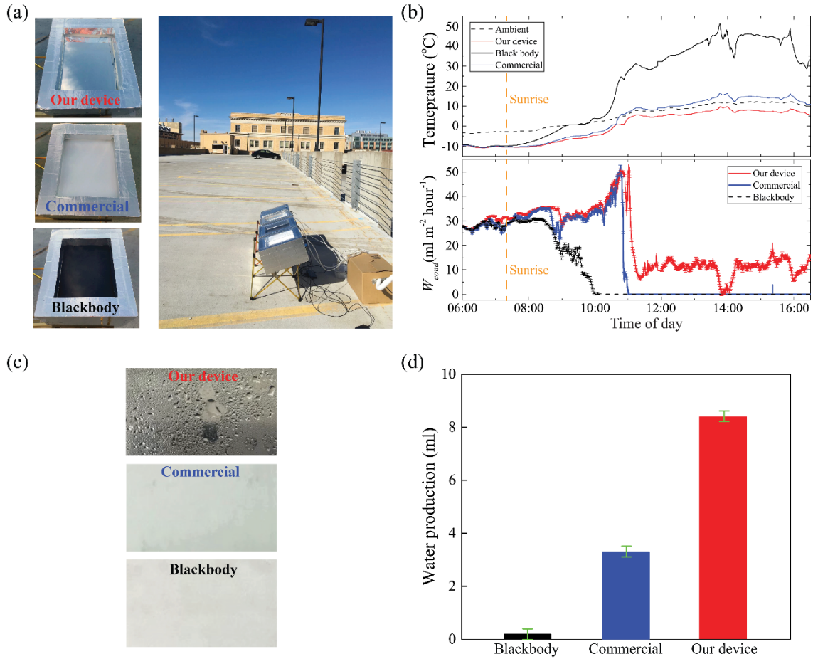
Figure 4. Experimental demonstration of daytime radiative condensation. (a) Left: front-side photographs of condensers used in our measurements. A blackbody and a commercial radiative dew condenser (OPUR foil) are used for comparison. Right: Outdoor experimental setup. The condensers are placed on the roof of a parking ramp at the University of Wisconsin – Madison, under direct sunlight. (b) Top panel: real-time temperatures of our daytime radiative condenser (red line), the commercial radiative condenser (blue line) and a blackbody (black line). The black dashed line represents the ambient temperature. Bottom panel: real-time condensation rates of our daytime radiative condenser (red line), the commercial radiative condenser (blue line) and a blackbody (black line). The condensation rates are measured relative to the convective condenser. The error of our temperature measurements is \pm 0.05 °C and the error of our relative humidity measurements is \pm 0.1\% . The error bars were calculated based on the measurement errors. The measurement was performed on March 11 th . The temperature of the blackbody was higher than the ambient temperature due to absorption of sunlight, and thus the blackbody had zero condensation rate. The temperature of the commercial condenser initially was below ambient temperature in the morning but increased to above ambient temperature around 11:00. Consequently, the condensation rate of the commercial condenser dropped to zero around 11:00. Conversely, our daytime condenser remained at a temperature lower than the ambient temperature and provided condensation throughout the day. (c) Photos of the condensing surface for each condenser taken around 17:00 on March 11 th . (d) Daily water production from dawn to sunset. The water condensed by the blackbody before sunrise was not completely evaporated during daytime, leaving a small amount of water in the condensing chamber.
