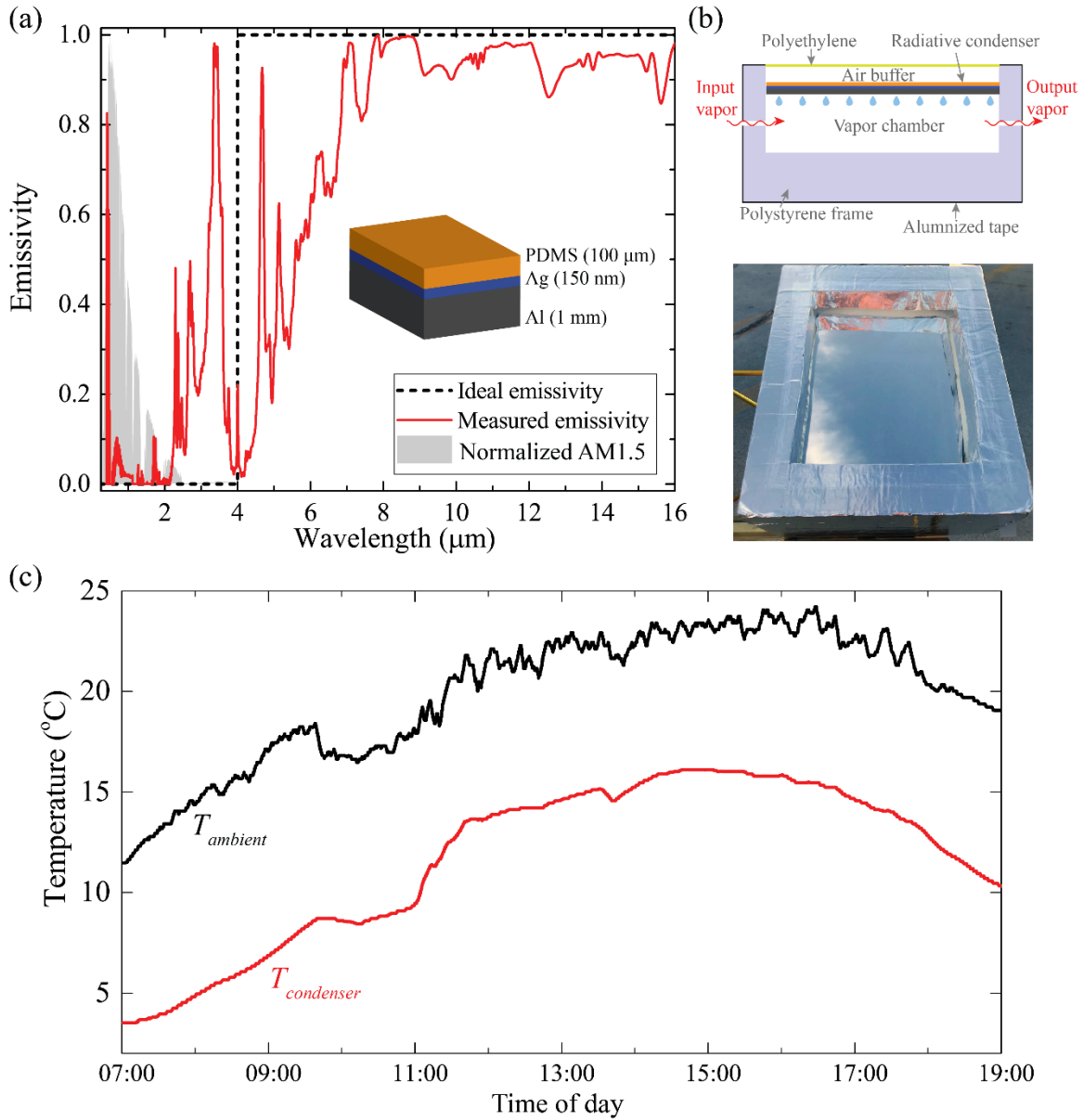
Figure 3. Experimental realization of our daytime radiative condenser. (a) Schematic of the daytime radiative emitter and the measured normal-incidence emissivity spectrum. The emitter consists of a 100- \mu\text{m} layer of PDMS, a 150-nm layer of silver, and a 1-mm-thick aluminum plate. (b) Experimental setup. The emitter is placed inside an insulating polystyrene box. The opening of the insulating box is covered by a thin polyethylene film and the external surface of the box is covered by aluminized-foil tape. (c) Measured temperature under direct sunlight, which is about 8 ^{\circ}\text{C} lower than the ambient temperature throughout the day. The measurement was performed on the roof of the Space Science and Engineering Building at the University of Wisconsin – Madison on September 29 th , 2017.
