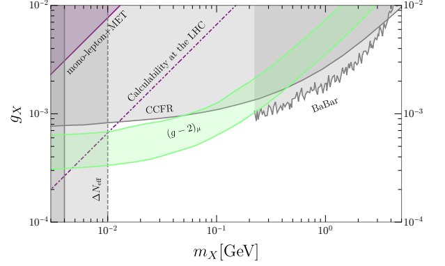
Figure 2. High mass constraints on a Stueckelberg U(1)_{L_\mu-L_\tau} gauge boson with Dirac neutrino masses. The solid and dot-dashed purple lines are the same as in Fig. 1. Other constraints are from: \Delta N_{\text{eff}} during BBN due to thermalization of A_X and entropy dump during its decay [35, 40, 41] (solid: T_{\text{RH}} > 4 MeV, see e.g. [42, 43]; dashed: T_{\text{RH}} > 10 MeV), neutrino trident process at the CCFR experiment [44, 45], and a search for e^+e^- \rightarrow \mu^+\mu^- A_X , A_X \rightarrow \mu^+\mu^- at BaBar [46]. In the shaded green region, the muon (g-2)_\mu can be explained by A_X at 2\sigma [9, 49].
