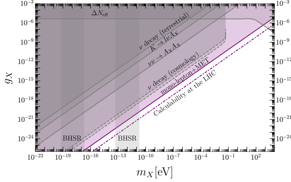
Figure 1. Low mass constraints on a Stueckelberg U(1)_{L_\mu-L_\tau} gauge boson with Dirac neutrino masses. The purple region shows the constraint derived in Eq. (19) coming from the high transverse mass tail of mono-lepton+MET events at the LHC. The dot-dashed purple line denotes the constraint obtained from demanding the validity of perturbation theory at the LHC, given by Eq. (20). Other constraints are from: \Delta N_{\text{eff}} during BBN through thermalized A_X [35], black hole super-radiance (BHSR) instability [36], rare K decays [22], \Delta N_{\text{eff}} through \nu\nu \rightarrow A_X A_X [22, 35], constraints on \nu decay through terrestrial experiments [22, 37, 38]. We also update the cosmological constraints on \nu decay as discussed in the main text, based on the recent result of Ref. [39]. Given the \nu decay bounds from cosmology are model-dependent and can be relaxed, we show it via dashed lines.
