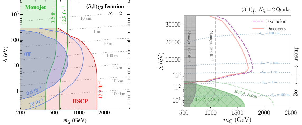
Figure 30: Recast limits on quirks from [331] (left) and projected limits on quirks from [332] (right).
