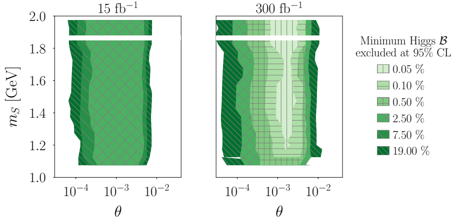
Figure 25: Exotic Higgs branching ratio excluded at the 95 % C. L at LHCb for a total integrated luminosity of 15 \text{ fb}^{-1} (left) and 300 \text{ fb}^{-1} (right) Results are presented for a model with a hadrophilic (leptophobic) S , following [264] (plot from Ref. [57]).
