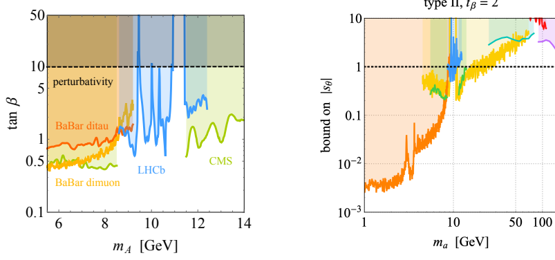
Figure 26: Left: 95% CL bounds on \tan \beta in the 2HDMII scenario. The blue, green, and orange curves follow from \Upsilon(n) production by LHCb [146, 269], a CMS dimuon resonance search [270], and the BaBar 90% CL limit on radiative \Upsilon(1) decays in the dimuon [271] and ditau [272] channels. The perturbativity bound on \tan \beta is also shown (black dashed). All shaded regions are excluded. For further details see Ref. [146]. Right: Limits on |s_\theta| in the 2HDMII+S with t_\beta = 2 . The green, blue and yellow regions are the same as in the left panel, while the additional turquoise, red, purple and brown exclusions correspond to the CMS searches for pp \rightarrow a b \bar{b} \rightarrow \tau^+ \tau^- b \bar{b} [273], pp \rightarrow a \rightarrow \gamma \gamma [274], pp \rightarrow a \rightarrow \tau^+ \tau^- [275] and the LHCb inclusive dimuon cross section [12]. The dashed black lines indicate |s_\theta| = 1 and coloured regions are excluded at 95% CL apart from the orange and yellow contours which only hold at 90% CL. For further details see Ref. [266].
