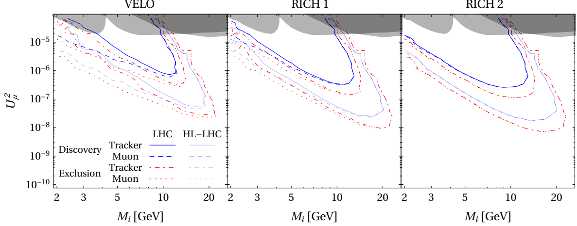
Figure 16: Comparison of the discovery (blue) and exclusions (red) reaches for HNLs with pure muon mixing U_\mu^2 at the LHCb detector with 13 and 14 TeV after collecting 30 and 380 fb ^{-1} of data. Here we assume that secondary vertices originating from HNL decays happening within the first half of the VELO or before the RICH 1 or 2 can be reliably identified. The dashed and dotted curves include muons identified only identified in the muon system.
