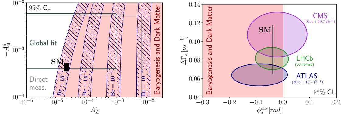
Figure 15: Left panel: Parameter space in the A_{\text{sl}}^d - A_{\text{sl}}^s plane. We show SM predictions from [182], current world averages [185], and results from global fits (UTfit) [192]. Right panel: Experimental landscape in the \Delta\Gamma_s - \phi_s^{\text{ccs}} plane. Current measurements from LHCb [193], ATLAS [194], and CMS [195] are shown. The regions highlighted in red allow for successful baryogenesis and dark matter production as described in the text.
