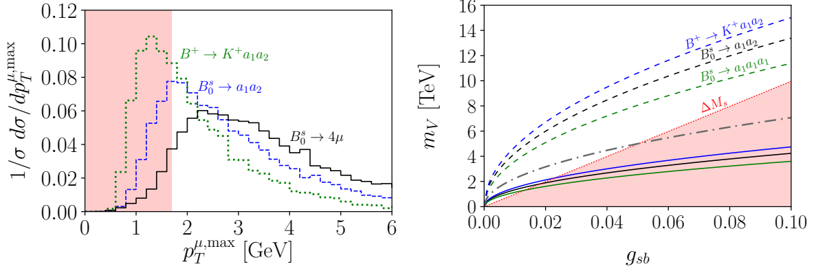
Figure 9: ( Left ) Normalized distribution of the transverse momentum of the hardest muon for B_0^s \rightarrow a_1 a_2 and B^+ \rightarrow K^+ a_1 a_2 , with m_1 = 1 GeV and m_2 = 2.5 GeV. These distributions are compared with that of B_0^s \rightarrow 2\mu^+ 2\mu^- . ( Right ) Maximum value of m_V that can be tested in the searches for B_0^s \rightarrow 3\mu^+ 3\mu^- and B^+ \rightarrow K^+ 3\mu^+ 3\mu^- at the current run of the LHCb (solid lines) and for Upgrade II (dashed lines). The red dotted line delimits the area excluded by measurements of \Delta M_s . In the dash-dotted line the anomalies in R_K and R_{K^*} can be explained at the 1\sigma level [138]. We have fixed g_{12} = 0.5 and m_1 = 1.2 GeV. We have set m_2 = 2.0 GeV for B_0^s \rightarrow a_1 a_2 and B^+ \rightarrow K^+ a_1 a_2 . For B_0^s \rightarrow a_1 a_1 a_1 , we have fixed instead m_2 = m_{12} = 5 GeV.
