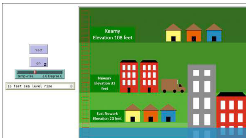
Figure 1: Sea level rise simulation
