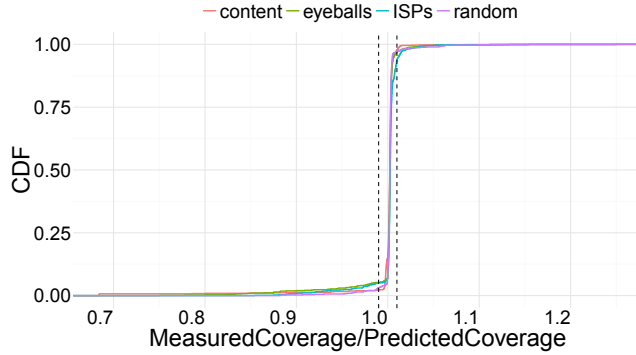
Fig. 14. The measured coverage of AS graphs obtained via running traceroutes is very close to the coverage predicted by BGP policy simulations. Therefore the approximate gain of a measurement used by the greedy algorithm is close the gain obtained by running the measurement.
