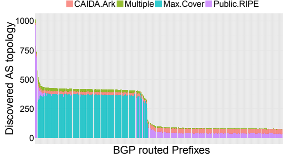
Fig. 15. Number of ASes in the empirically derived directed acyclic graphs (DAGs) for each prefix. Prefixes are ranked by the number of AS included in the DAG and prefixes with less than 75 ASes in their graph are not shown, they are qualitatively similar to the ASes on the right-hand side of the graph.
