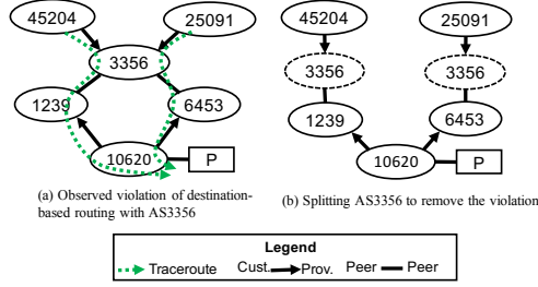
Fig. 4. Example of violation of destination-based routing. Depending on the prior hop AS 3356 (Level 3) selects a different next-hop towards the destination. Splitting this node produces a tree-structured prefix DAG.
