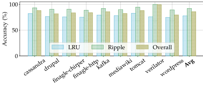
Fig. 10: Ripple 's accuracy for different applications: On average Ripple provides 92% accuracy which ensures that the overall accuracy is 86% even though underlying LRU has an accuracy of 77.8%.
