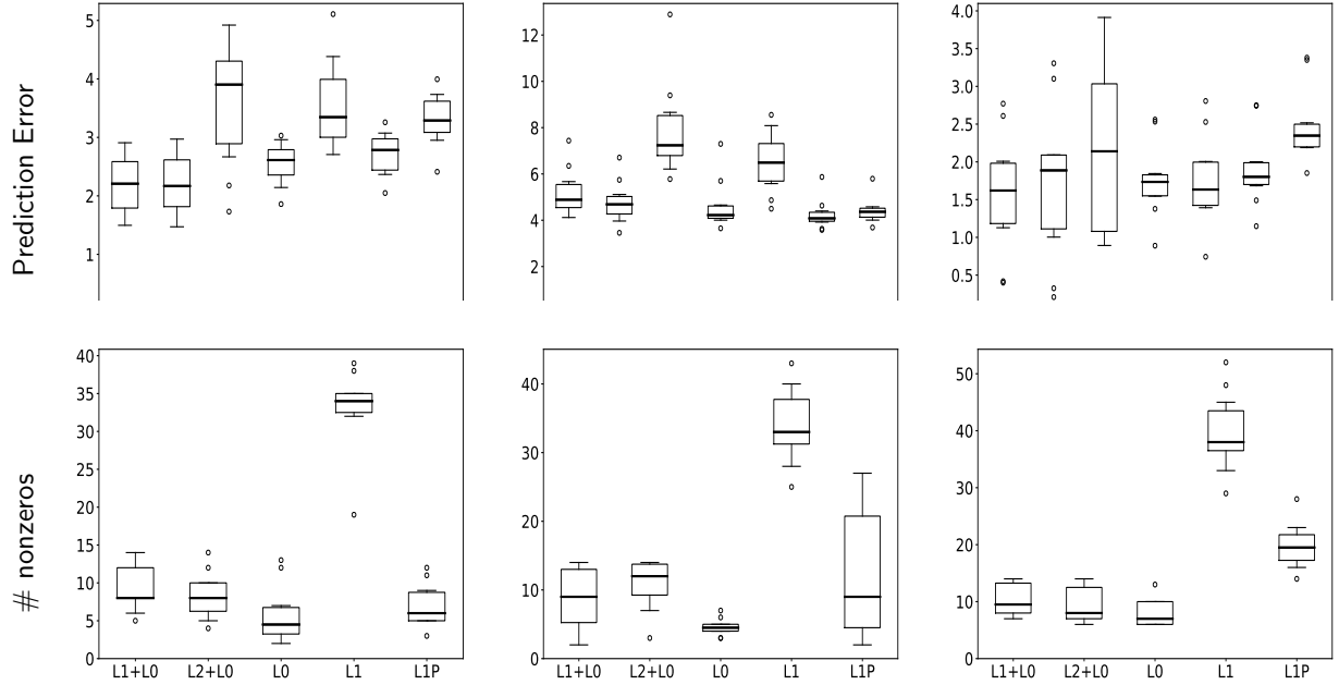
Figure 3: Experimental results for Example 2. The results are qualitatively similar to Figure 2 – however, this example is “harder” than Example 1 due to the increased correlation among the features – a larger nominal value of SNR is required before L0 matches the performance of L0+L1/L0+L2. The L0+L1/L0+L2 methods performed the best in terms of obtaining a good predictive model that is also sparse – the model sizes were larger than k^* but smaller than those available from the best L1 models.
