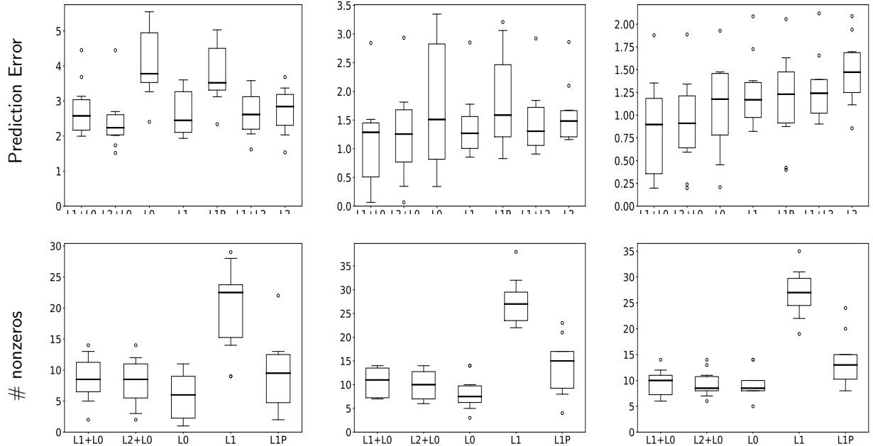
Example 1: Large settings: n = 100, p = 1000
