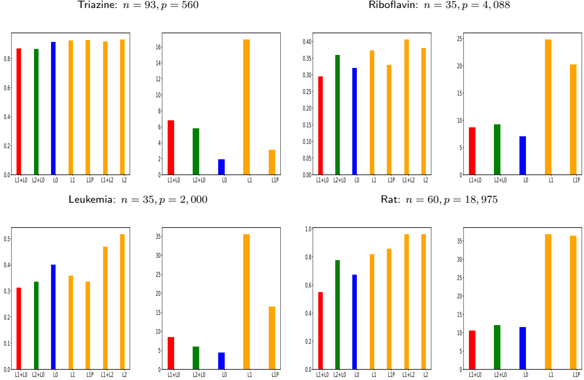
Figure 5: Performance of the methods on four real datasets. We observe that pure L0 tended to underfit by selecting models that are overly sparse. L0+L1/L0+L2 worked well both in terms of prediction and in terms of sparsity, when compared to the best available L1 models. L1 led to models with good predictive accuracy, but at the cost of a significant increase in density.
