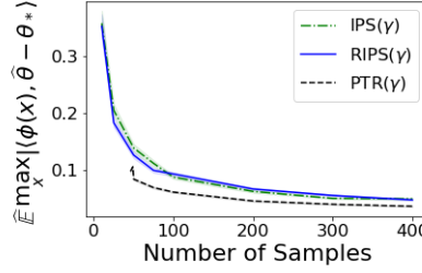
Figure 3. Kernel Experiment
