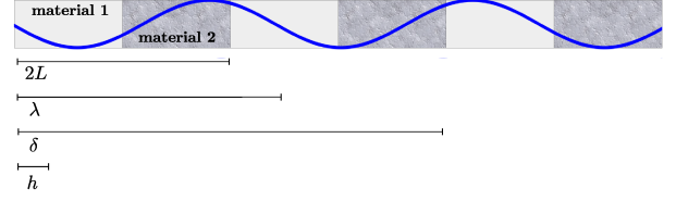
Figure 1: One-dimensional bar with ordered microstructure of period 2L . Material 1 and 2 have the same density and Young modulus E_1 and E_2 . The horizon \delta , the wave length \lambda , and the discretization size, h , are reported for comparison.
