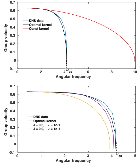
Figure 5: Comparison of the group velocity. Upper: group velocity corresponding to K_{\text{opt}} , K_{\text{const}} , and DNS data. Bottom: group velocity corresponding to K_{\text{opt}} for different pairs (\delta, \epsilon) .
