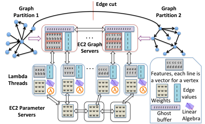
Figure 2: Dorylus’s architecture.
