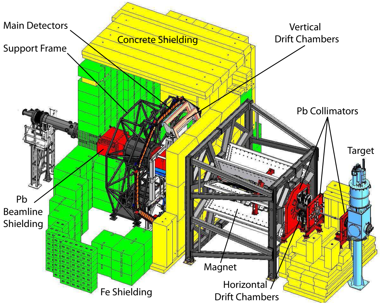
FIG. 1. CAD view of the experimental apparatus, which reveals more otherwise hidden details than a photograph can. The beam was incident from the right. The key elements include the target scattering chamber (cyan), a triple collimator system (red), a resistive eight-fold symmetric toroidal magnetic spectrometer (grey), and eight Cherenkov detectors (narrow dark orange octagonal ring in an azimuthally-symmetric array around the beamline at a radius of 3.4 m). Two tracking drift chambers are illustrated just upstream of the eight Cherenkov detectors; the latter are arrayed about the beamline 12.3 m downstream of the target. For clarity, only some portions of the extensive steel and concrete shielding are shown.
