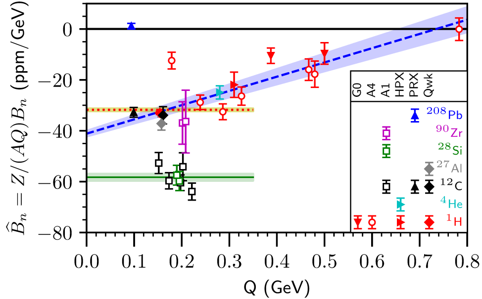
FIG. 8. World transverse asymmetry data B_n are scaled by the factor Z/(AQ) and plotted against Q (in GeV). Symbols and colors are as in Fig. 7. The dotted red and solid green lines represent fits to the intercepts of the Group 1a & 2 data, respectively, and thus correspond to the slopes \widehat{B}_n in Fig. 7 and Table VII. The blue dashed line is a linear fit to all the Group 1 data, corresponding to the quadratic fit in Fig. 7 and Table VII. Uncertainties in the fits are denoted by the bands in the figure.
