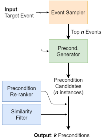
Figure 1: The DiP pipeline. Candidates are generated conditioned on the Event Sampler. The Re-ranker and Similarity Filter improve quality/diversity.
