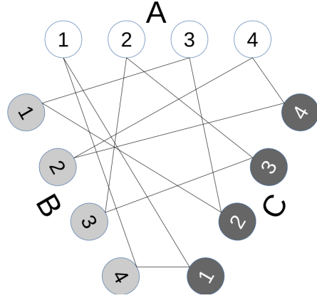
Figure 1: n = 4 3D matching with matches \{141, 233, 312, 424\}
