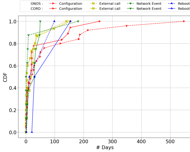
Figure 7: CDF of Resolution Time for Triggers.
