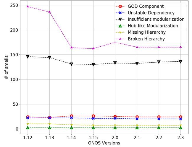
Figure 8: Distrubution of Six Code Smells. A: God Component, B: Unstable Dependency, C: Insufficient Modularization, D: Hub-like Modularization, E: Missing Hierarchy, F: Broken Hierarchy in ONOS Cores Versions.
