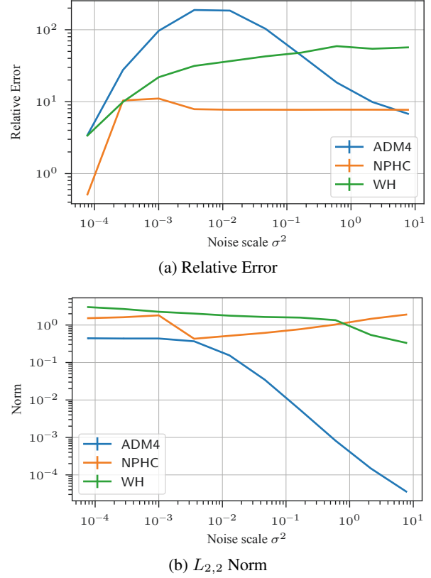
Figure 7: Sensitivity analysis of the estimation to noise scale for the Bund Futures traded at Eurex.
