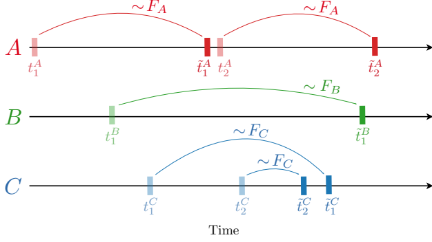
Figure 2: An example of events in a three-dimensional point process and their translations. Events in dimension A , (resp., B and C ) are translated randomly by F_A (resp., F_B and F_C ).
