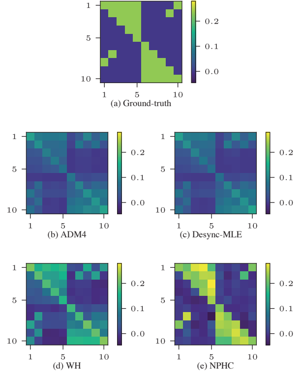
Figure 4: Comparison of the integrated kernel matrix estimated by several methods under noisy observations.
