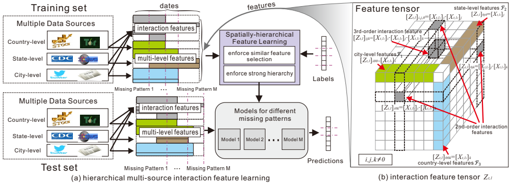
Fig. 3. A schematic view of hierarchical incomplete multi-source feature learning (HIML) model.
