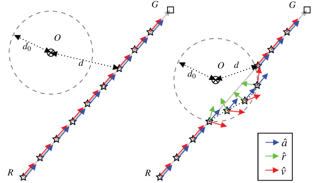
Fig. 4: Example trajectories of a robot around an obstacle using the proposed approach. The repulsive potential \hat{r} affects the robot only if d \leq d_0 . The position of object O is represented by a cross, the goal position G by a square, and the position of robot R over time with stars. (left): when the obstacle is not along the direct path from the robot to the goal, it does not affect robot navigation. (right): the robot's direct path to the goal brings it closer than d_0 distance to the obstacle; our algorithm forces the robot to circumnavigate around it.
