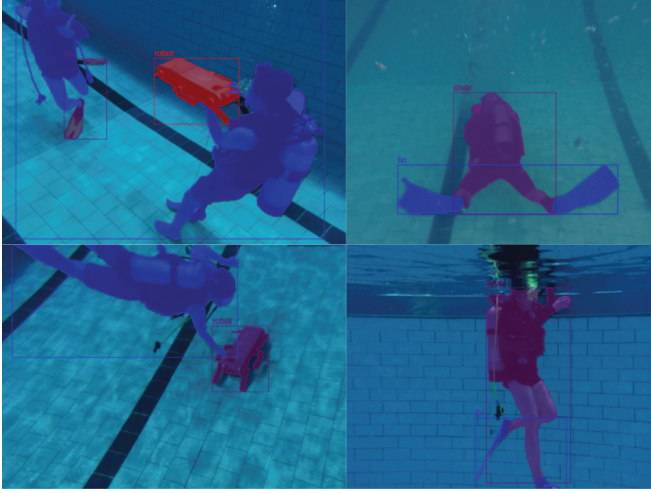
Fig. 3: Examples of labeled training images from our underwater dataset showing three classes: diver , robot , and fin (the colors for each class are randomly selected per image).
