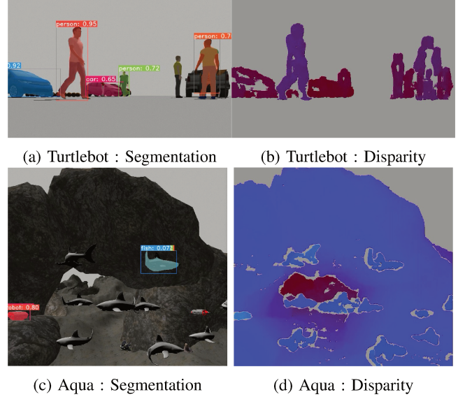
Fig. 6: Instance segmentation and disparity estimation from the view of robots. Fig. 6a and 6b are captured from the Turtlebot in the terrestrial world, and Fig. 6c and 6d are from the Aqua robot in the underwater world.
