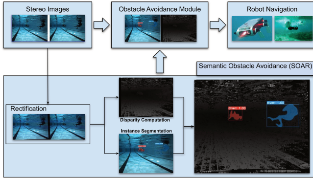
Fig. 2: Illustration of our obstacle avoiding approach which fuses depth and semantic information for selective avoidance. The input is a pair of stereo images, which is used to both compute disparity and, through YOLACT, generate semantic labels for obstacles in the scene. Fusing these, a robot has both depth estimates and semantic information about potential obstacles, enabling it to select navigation strategies depending on the nature of the obstacle.
