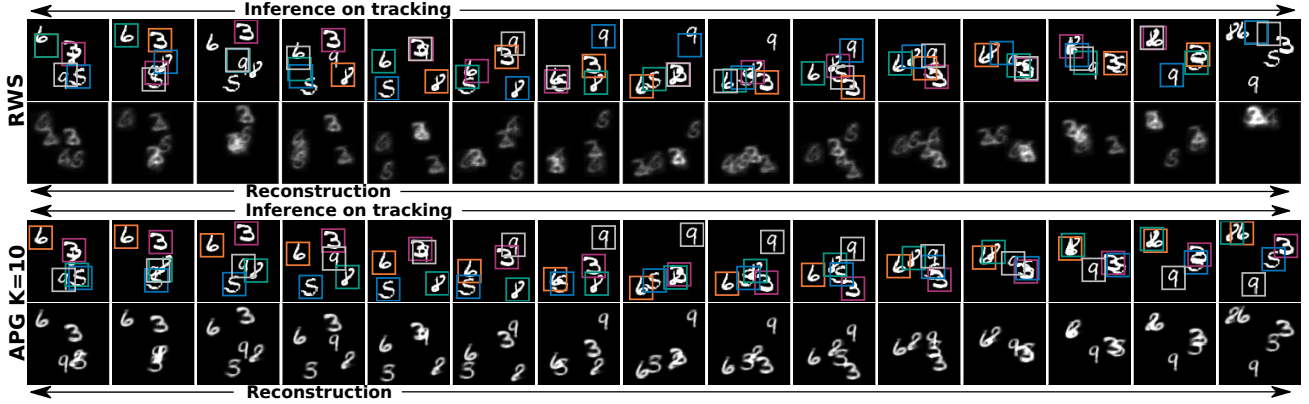
Figure 4. A single sample from variational distribution in one video instance with T = 100 time steps and D = 5 digits. The visualization is truncated to the first 15 time steps due to limited space (see Appendix I for full time series and Appendix H for more examples). The sample is initialized from RWS (top) and updated by K = 10 APG sweeps (bottom). The APG sampler improves the inference results in tracking and learns better MNIST digit embeddings that improve reconstruction.
