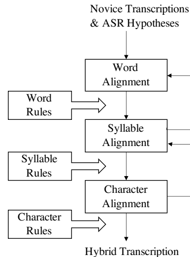
Figure 1: Novice-ASR Fusion Process
