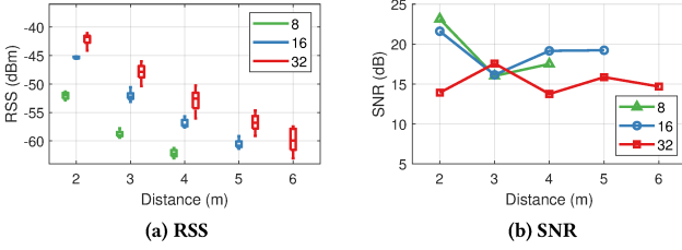
Figure 15: Impact of radar-to-tag distance.
