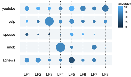
Figure 7: The coverage and accuracy of our used labeling functions on five datasets. Larger circle denotes higher coverage and lighter color denotes higher accuracy.
