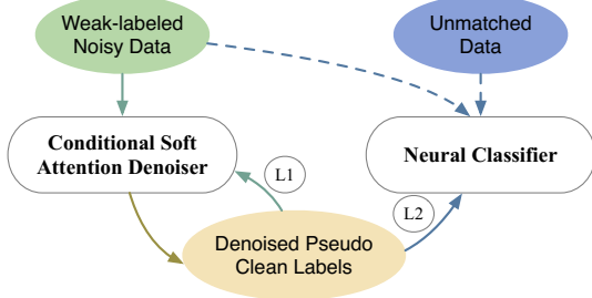
Figure 2: Overview of cross-training between the rule-based classifier and the neural classifier.
