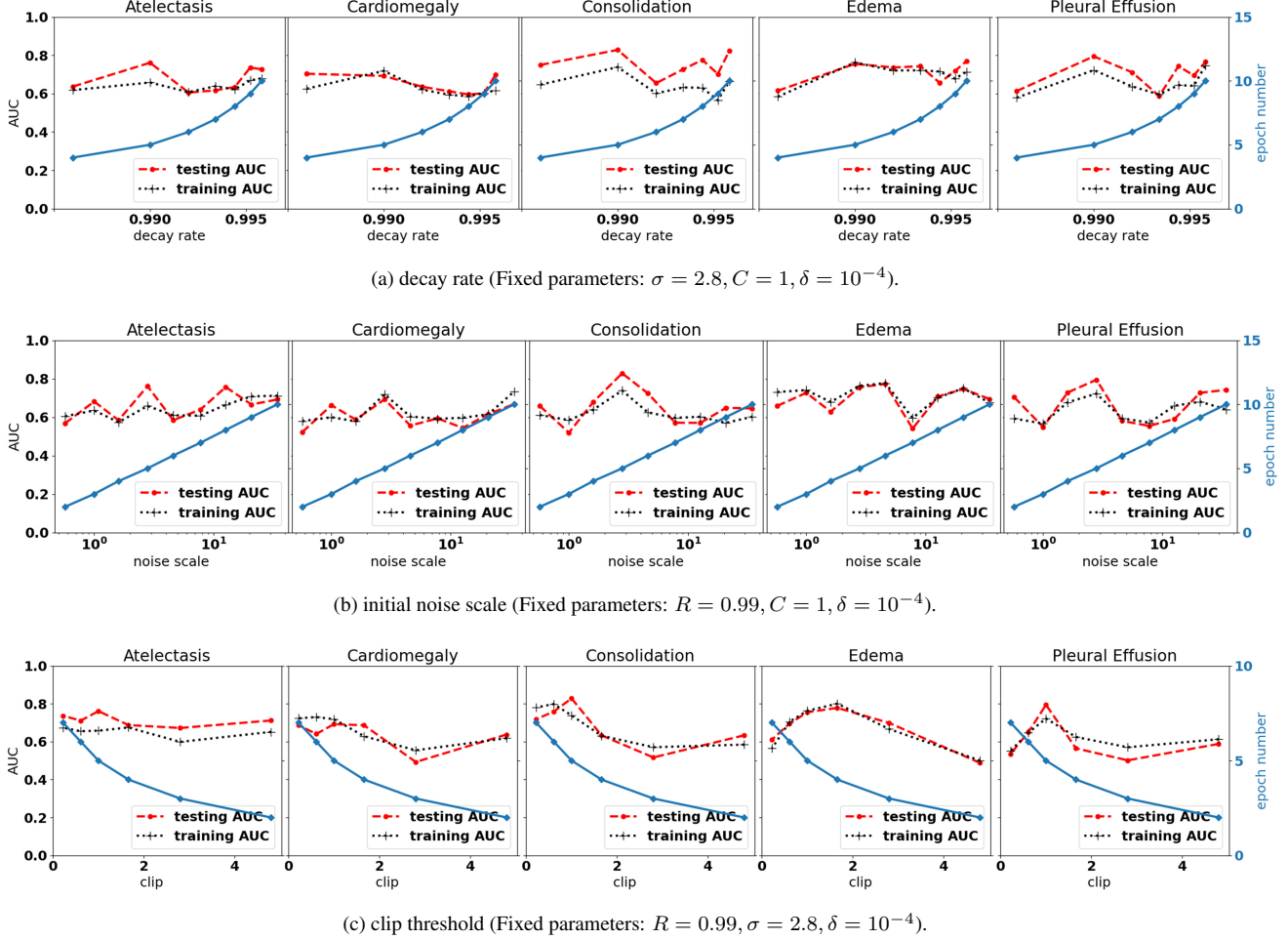
Figure 2: The impact of parameters on the training model performance (Red curve is testing AUC, black curve is training AUC and the blue curve is epoch number).
