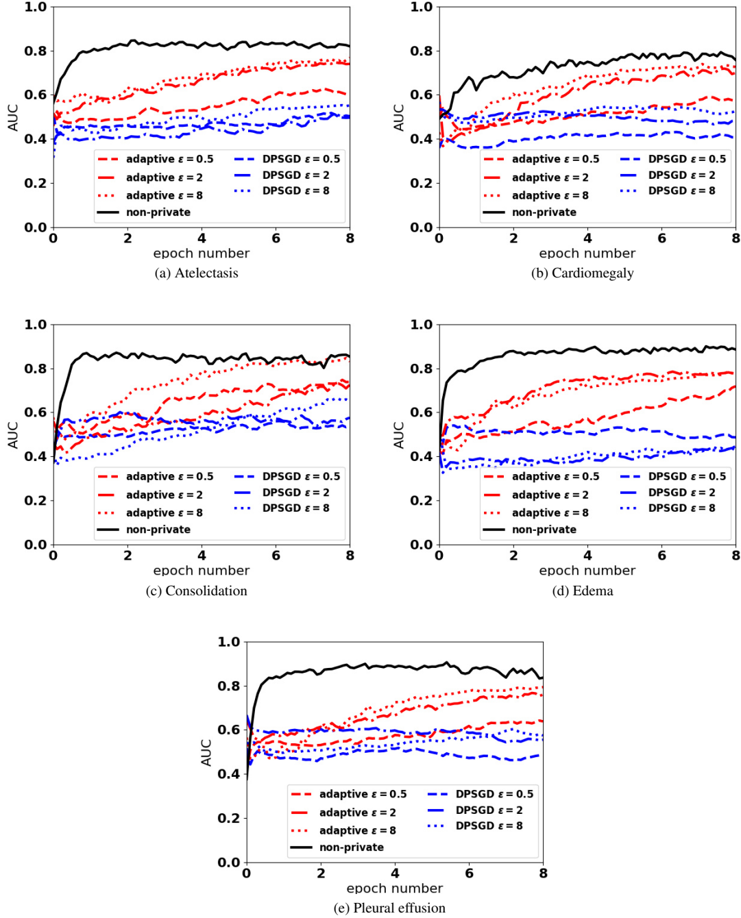
Figure 1: Comparison between non-private model, DPSGD and our adaptive DP model.
