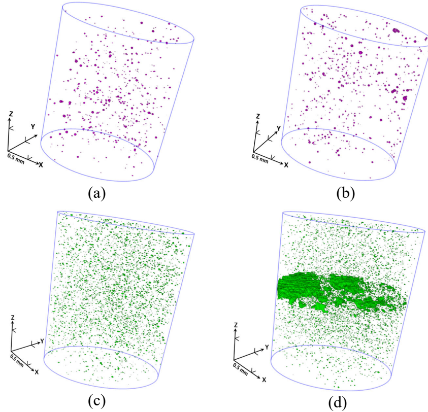
Figure 3. X-ray tomography images comparing the internal porosity of a (a) default and (b) 2-layer modified thickness 316L SS specimen, as well as (c) default and (d) 2-layer modified thickness 17-4PH SS specimen near/at the cross-section volume [24].
