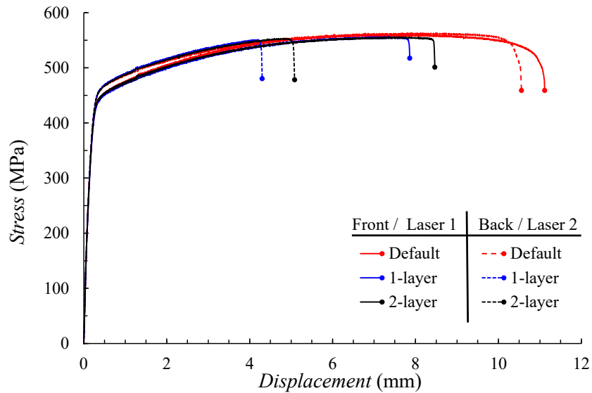
Figure 4. Stress vs. displacement curves comparing the tensile deformation behavior of default, 1-layer, and 2-layer LB-PBF 316L stainless steel specimens fabricated using a GE Concept Laser M2 dual laser AM system.
