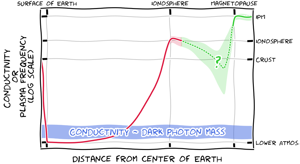
FIG. 1. Sketch of the conductivity (or plasma frequency, where applicable) profile in the vicinity of the Earth's surface in (1) the case where the ionosphere is thick enough to damp active photon modes [solid red], and (2) the case where it is not and we must consider the electrical environment out to the interplanetary medium (IPM) [dotted and solid green]. In the former case, we terminate the sketch some distance into the ionosphere, as the details above that altitude are irrelevant. In the latter case, we note that the conductivity or plasma frequency in the magnetospheric region (i.e., between the ionosphere and the magnetopause) can be quite complicated, and we have indicated this by dotting the green line, and including the shaded band and the question mark: we show in Sec. III C that, under reasonable assumptions, the details of the profile here do not matter for our signal. The vertical extent of the blue band indicates the range of dark-photon masses m_{A'} we consider, in correct relation to the relative sizes of (a) the conductivity in the lower atmosphere, (b) the conductivity in the Earth's crust/upper part of the mantle (representative value labeled on the plot), (c) the conductivity of the ionosphere, and (d) the plasma frequency of the interplanetary medium beyond. While we stress that this plot is highly schematic, it correctly captures that, in the upper atmosphere (interplanetary medium) and the Earth's crust, the conductivity (plasma frequency) exceeds the dark-photon mass, while the opposite is true in the lower atmosphere. The reader is referred to the text of Sec. II B for detailed discussion and caveats associated with this sketch.
