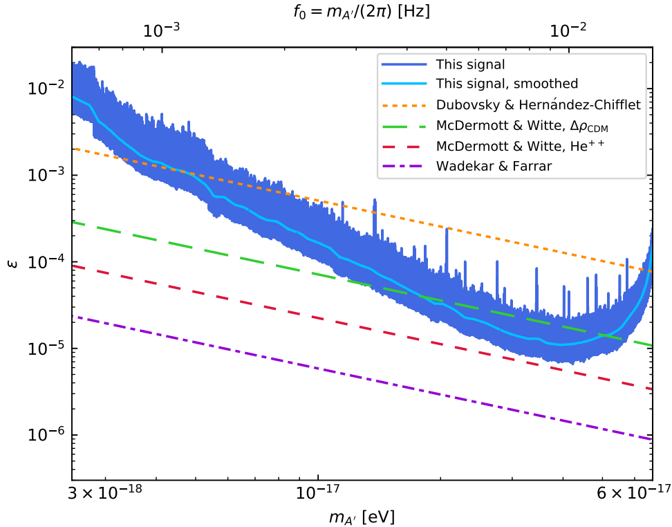
FIG. 4. The 95%-credible upper limits on the kinetic mixing parameter \varepsilon that result from the experimental search outlined in Sec. IV (and to appear in Ref. [38]) are shown as the dark blue line as a function of the dark-photon mass m_{A'} (the line appears as a band owing to the density of frequencies at which limits are plotted, and fluctuations of the limits from one frequency to the next). The sliding average of these limits over nearby frequencies are shown as a lighter blue line as a guide to the eye. These limits assume that the dark photon is all of the dark matter. Also shown are a variety of existing astrophysical limits arising from heating effects of dark-photon dark matter on gas in various astrophysical settings: the ionized interstellar medium in the Milky Way (dotted orange) [34]; the intergalactic medium around helium reionization (short-dashed red, labeled ‘ \text{He}^{++} ’) [40]; and gas in the Leo T dwarf galaxy (dot-dashed purple) [41]. We also show a DM-depletion limit from non-resonant dark-photon-photon conversion [40] (long-dashed green, labeled ‘ \Delta\rho_{\text{CDM}} ’).
