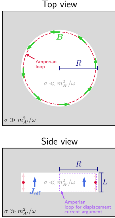
FIG. 2. Schematic view of the toy example cylindrical cavity of poorly conducting material (white) of radius R and height L \ll R hollowed out of a good conductor (gray). Also shown are (1) the Ampèrian loop discussed in the text (red dashed in top view; red markers in side view), which can be located anywhere within the vertical height of the cavity along the short dimension (as indicated by the pink arrows); (2) the effective current \mathbf{J}_{\text{eff}} (blue arrows in side view), assuming that the dark-photon field is perpendicular to the top and bottom surfaces of the cavity; (3) the induced observable magnetic field \mathbf{B} (green arrows in top view); and (4) the Ampèrian loop (dotted purple in the side view) that we consider for the argument which we advance in footnote 11 that the displacement current can be ignored (this loop runs along a straight ray emanating from the center of the cavity in the top view).
