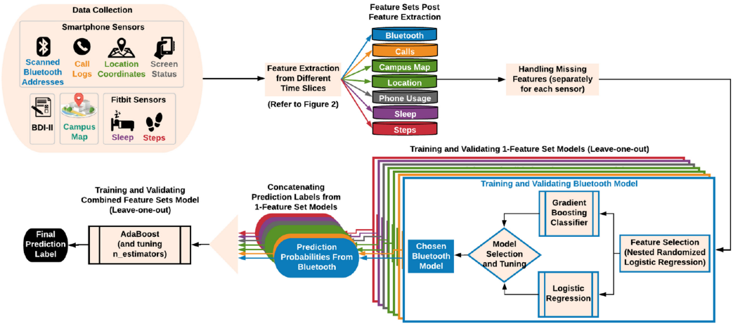
Fig. 1. Pipeline for the data processing and analysis.
