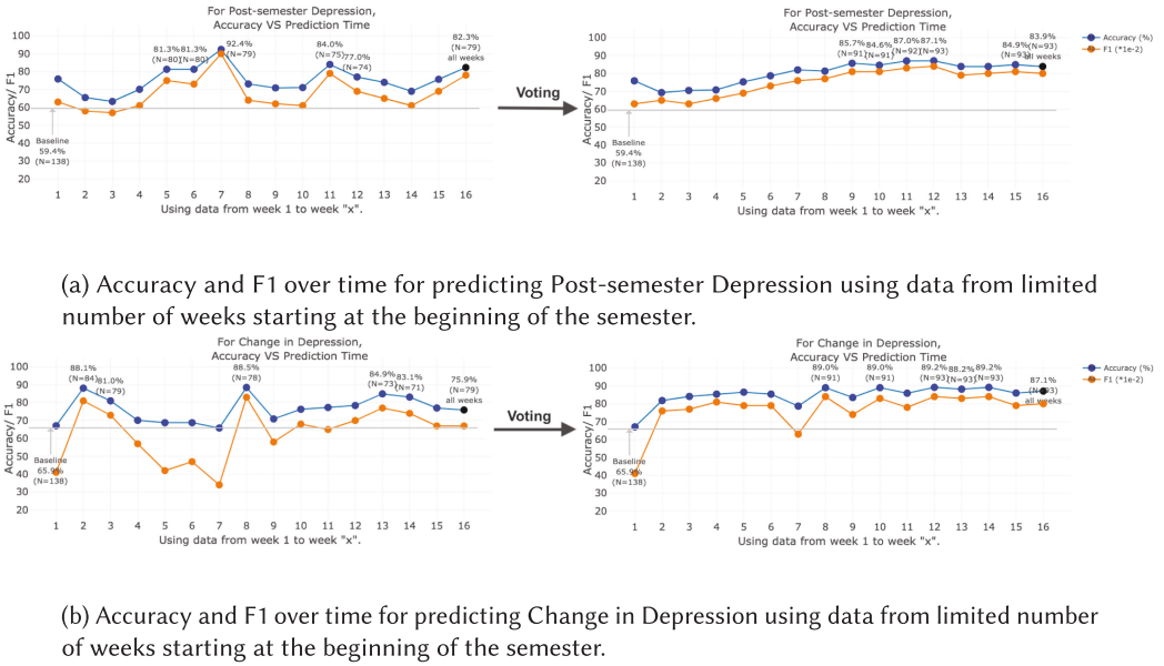
Fig. 5. Accuracies over time obtained when predicting (a) Post-semester Depression and (b) Change in Depression using data from a limited number of weeks starting at the beginning of the semester (week 1–week x ). In the graphs on the left side, for each time step, detections from all available feature sets are combined to get the corresponding accuracy. In the graphs on the right side, at time step x , majority voting is used on predictions from models at weeks 1– x (shown on the left) to obtain more stable performance across the 16 weeks.
