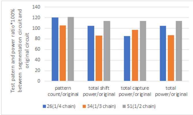
Fig. 3. fm_receiver Total test power for transition fault patterns with regard to pattern count for different amounts of scan chain segmentation
