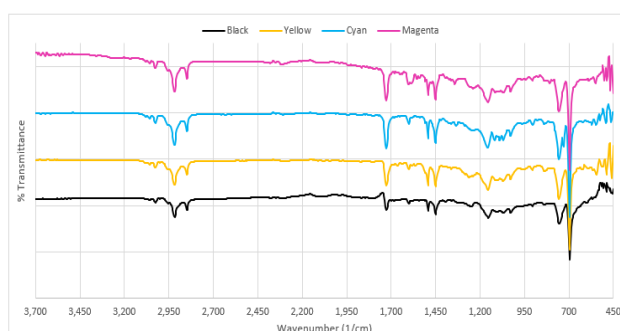
Figure 7. FTIR spectra from the laserjet ink samples
