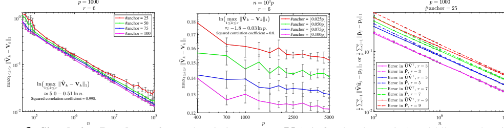
Figure 3: Simulation Results. Left: Total variation error on \mathbf{V} ( p is fixed and n varies). Middle: Total variation error on \mathbf{V} ( p/n is fixed). Both panels validate the scaling of \sqrt{p/n} in Theorem 3. Right: Recovery error of \mathbf{P} , where \hat{\mathbf{U}}\hat{\mathbf{V}}^\top is our method and \bar{\mathbf{P}} is the spectral estimator [37] (note: this method cannot estimate \mathbf{U}, \mathbf{V} ).
