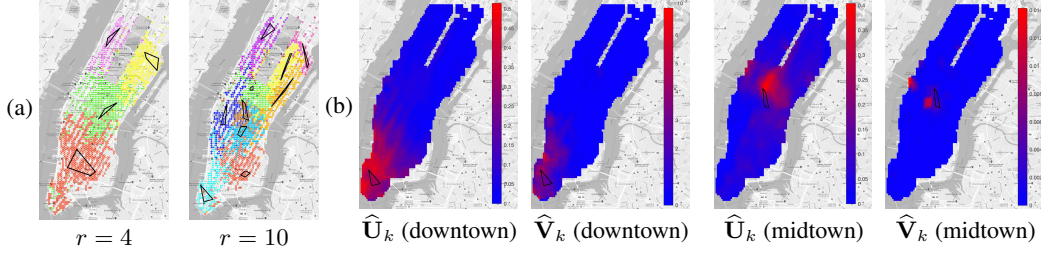
Figure 4: State aggregation results. (a) Estimated anchor regions and partition of NYC. (b) Estimated disaggregation distribution ( \hat{\mathbf{V}}_k ) and aggregation likelihood ( \hat{\mathbf{U}}_k ) for two meta-states.
