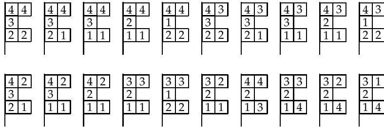
Figure 4: The semi-standard key tabloids of shape (0, 2, 1, 2) .
