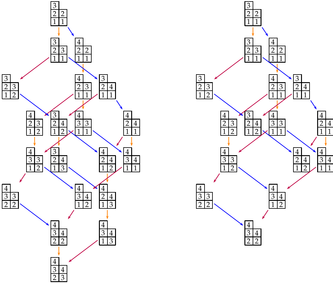
Figure 2: The crystal \mathcal{B}(2, 2, 1, 0) (left) and the Demazure crystal \mathcal{B}_{2431}(2, 2, 1, 0) (right), with edges f_1 ↙ , f_2 ↓ , f_3 ↘ defined by the lowering operators.
