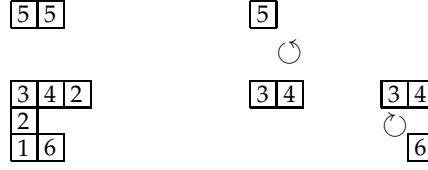
Figure 3: A non-attacking filling of the diagram for (2, 1, 3, 0, 0, 2) with the two co-inversion triples noted to the right.
