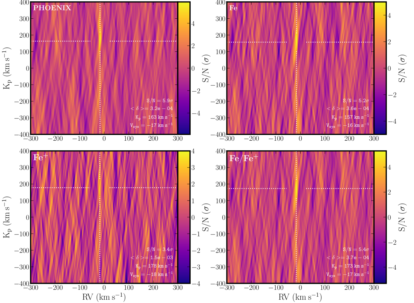
Figure 9. Atmospheric detections in TOI-1518b and their K_p - V_{sys} maps. The top-left corner of each panel indicates the cross-correlation template, and the bottom right corner lists properties of the peak value, including S/N of the detection, the average absorption depth after co-adding CCF rows ( \langle \delta \rangle ), and the maximal value of K_p , and V_{sys} . In all panels the Doppler shadow has been corrected per the methods in Section 3.2. For reference, we show results from cross-correlation with the PHOENIX spectrum used to model the Doppler shadow, revealing there are species common to both the planet’s atmosphere and star. The subsequent panels show results from cross-correlating with templates containing Fe and Fe + . In each panel, the white dotted lines indicate the K_p and V_{sys} with the highest signal.
