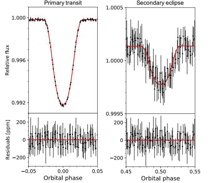
Figure 4. Zoomed-in views of the primary transit (left) and secondary eclipse (right) of TOI-1518b. The light curves are binned in 3-minute intervals. Note the difference in vertical scale between the two plots. The difference in out-of-occultation baselines primarily reflects the planetary phase-curve modulation. The bottom panels show the corresponding residuals from the best-fit model.
