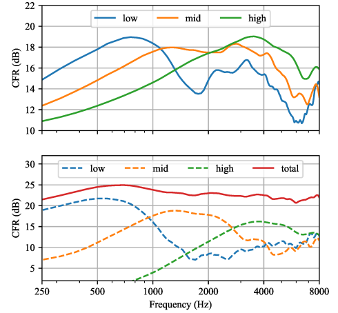
Figure 3: Top: CFRs of the learned filters at different scales of the single-scale waveform encoder. Bottom: CFRs of the learned filters of the multi-scale waveform encoder and its single-scale branch.
