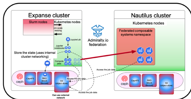
Figure 2: Expanse Composable Systems Architecture
