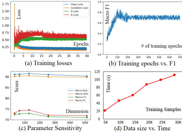
Figure 6: Stability, parameter sensitivity and scalability.
