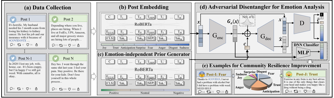
Figure 3: The overview of our proposed framework DR.Emotion.
