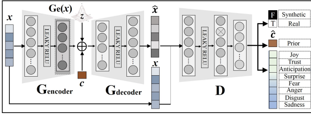
Figure 4: The framework of adversarial disentangler.
